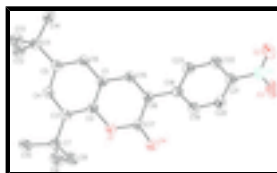
Fig. 1. The molecular structure of the title compound, showing the atomic numbering scheme. Displacement ellipsoids are drawn at the 30% probability level. Hydrogen atoms are omitted for clarity.
